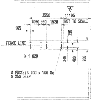
PLANER FOUNDATION DETAIL
